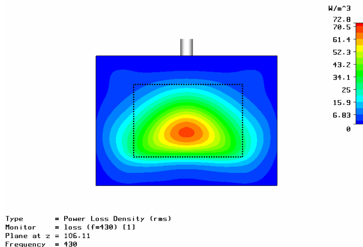
Fig. 6: Computation of effective aperture of SME applicator.
