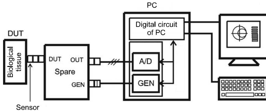
Fig. 1: Measurement circuit
