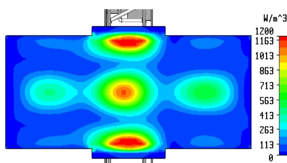
Fig. 2: SAR distribution after change of the position of connectors, case of 4 radiating elements.
