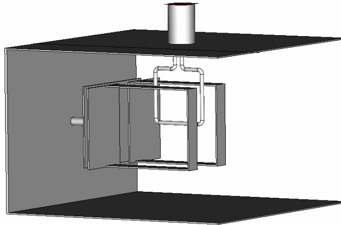
Fig. 4: Stripline applicator with Magnetic Excitation.
